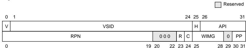
Figure 31. Page Table Entry Format—32-Bit Implementations
